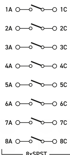
PK01-002 Switching Architecture
