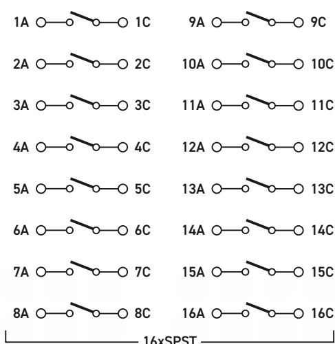
PK01-004 Switching Architecture
