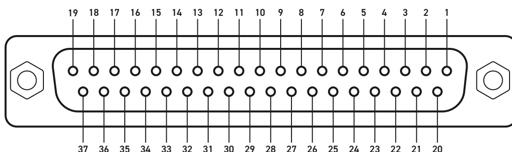
37-pin Female D-type Connector as viewed from front of module
