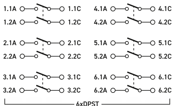
PK01-007 Switching Architecture
