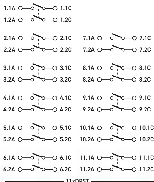
PK01-009 Switching Architecture
