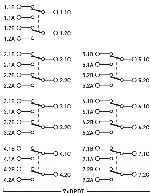
PK01-011 Switching Architecture
