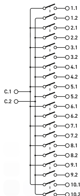
PK02-002 Switching Architecture
