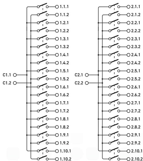
PK02-003 Switching Architecture
