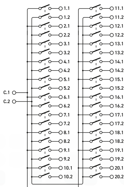
PK02-006 Switching Architecture
