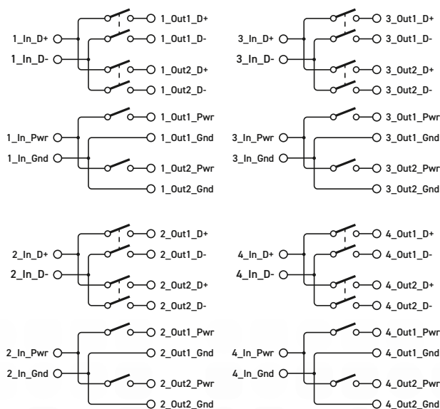
PK02-007 Switching Architecture
