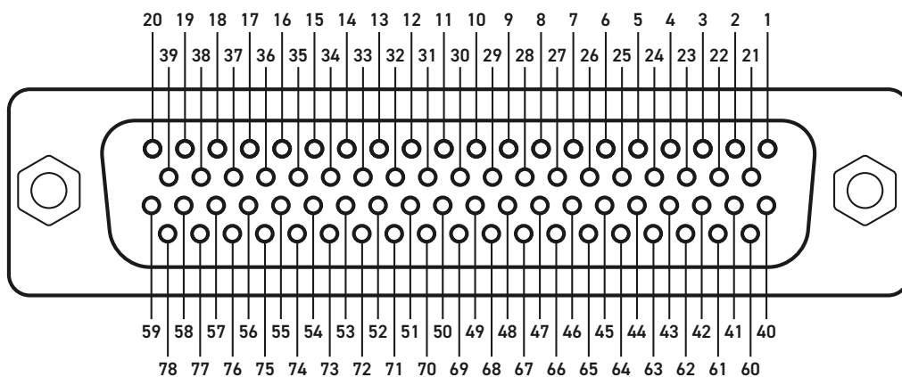
78-pin Female D-type Connector as viewed from front of module
