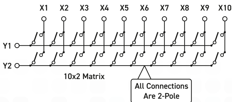
PK03-003 Switching Architecture
